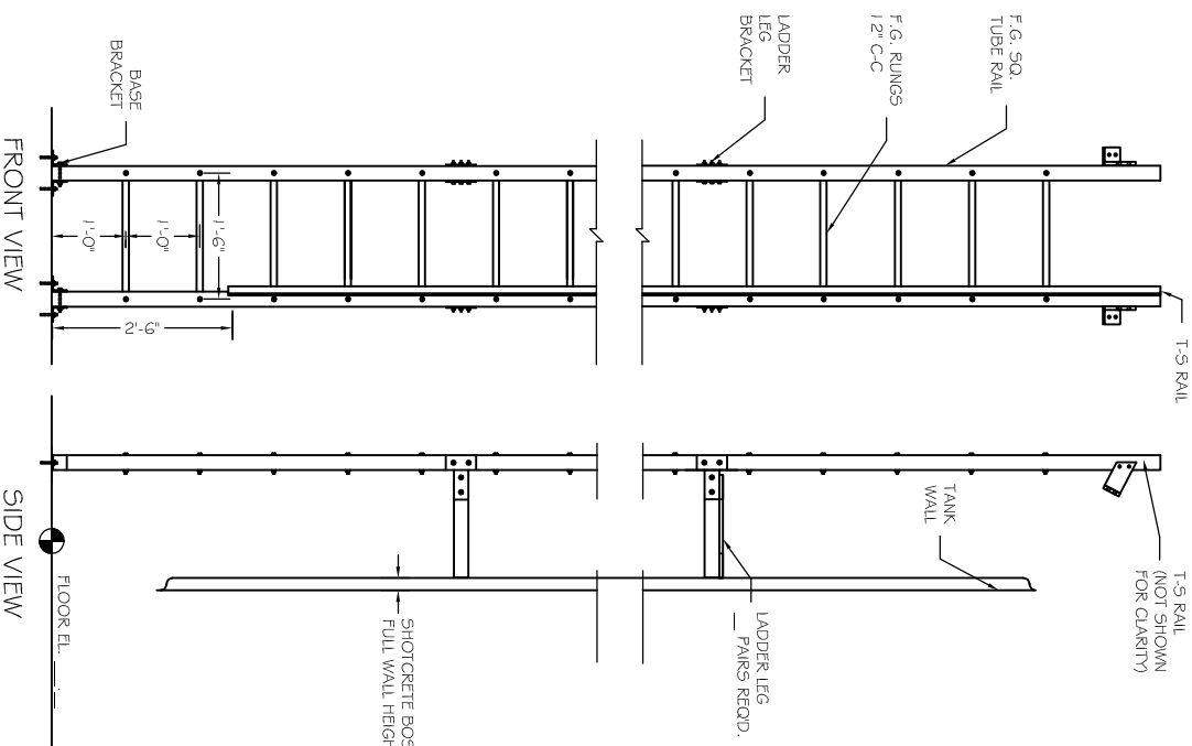
INTERIOR LADDER w/ T-S RAIL (RAIL REQUIRED OVER 20 FEET) NTS
