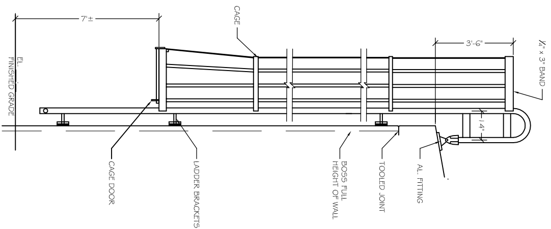
EXTERIOR LADDER WITH SAFETY CAGE (CAGE REQUIRED OVER 20 FEET) NTS
